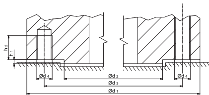
Part-turn actuator
